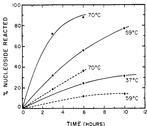
FIGURE 5: Reaction rates of CMP with malonyl hydrazide as a function of temperature. Reaction mixture contained 2 \times 10^{-4} M [2^{14}\text{-C}] CMP and 2 M malonyl hydrazide at pH 4.2. Reaction mixtures were analyzed by chromatography on Whatman 3MM paper in isopropyl alcohol-ammonia-water (7:2:1) and scanned. After incubation a new peak with lower mobility, representing the addition product, appeared (solid lines). At the higher temperature an intermediate peak appeared representing presumably a breakdown product (broken lines).
