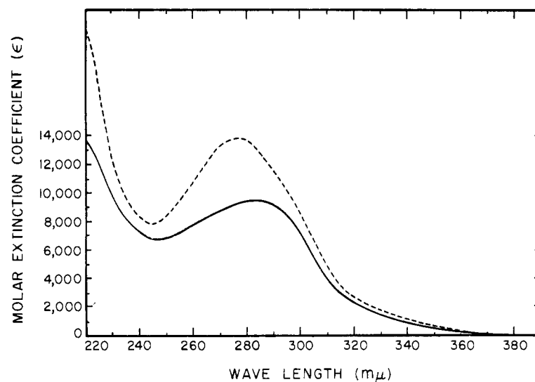
FIGURE 7: Ultraviolet absorption spectrum of the addition product of CMP with malonyl hydrazide (purified by electrophoresis) in 0.01 N HCl (pH 2). (—) addition product and (---) unreacted CMP.
