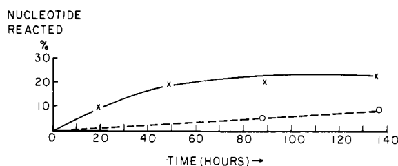
FIGURE 8: Reaction rate of CMP with DCBH. Reaction mixture contained 3 \times 10^{-4} M 2\text{-}^{14}\text{C} labeled CMP in 0.12 M DCBH at pH 4.2. Reaction mixtures were incubated at 37° and analyzed by paper electrophoresis at pH 7 where a faster moving peak is observed. A breakdown product (interrupted line) which does not move in electrophoresis forms at the same rate as the addition product.
