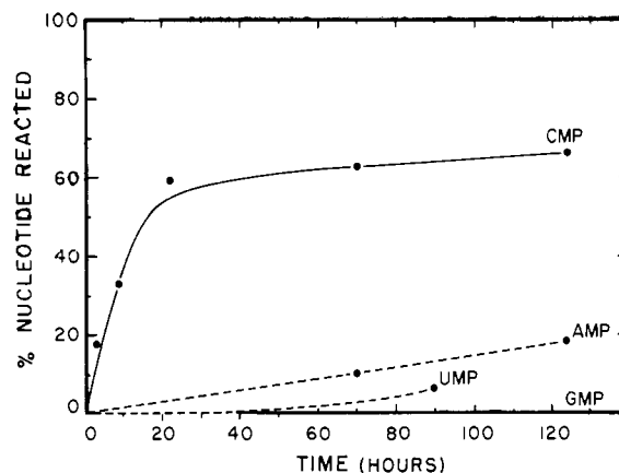
FIGURE 3: Reaction rates of ribose nucleotides with malonyl hydrazide. Reaction mixtures contained 2 \times 10^{-4} M ^{14}\text{C} -labeled nucleotides, 2 M malonyl hydrazide, at pH 4.2 incubated at 37^\circ . Aliquots were analyzed by paper electrophoresis and chromatography. Addition products are formed only with CMP (solid line). After 18 hr the reaction nearly stops. AMP, GMP, and UMP formed no addition products. After long times with UMP and AMP spots appeared which did not move in electrophoresis (broken lines).
