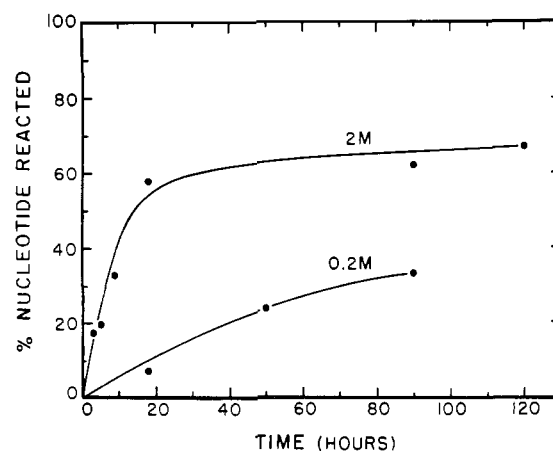
FIGURE 6: Reaction rate of CMP with malonyl hydrazide as a function of malonyl hydrazide concentration. Reaction mixtures contained 2 \times 10^{-4} M CMP and 2 and 0.2 M malonyl hydrazide at pH 4.2, respectively. The reaction mixtures were incubated at 37° and analyzed by paper electrophoresis at pH 7. The decrease in rate of reaction observed at the higher concentration is not observed at 0.2 M malonyl hydrazide.
