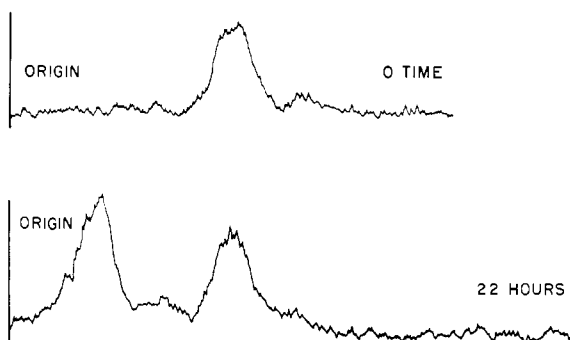
FIGURE 2: Scan of radioactivity of electrophoretic chart of same reaction mixture as in Figure 1. The buffer pH was 6.8. The greater mobility of the product than of the nucleotide suggests a greater negative charge presumably because of the added carboxyl group.
