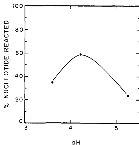
FIGURE 4: Dependence on pH of the reaction rate of CMP with malonyl hydrazide was measured by the extent of reaction after 20 hr at 37°. Content of reaction mixtures and analysis as in Figure 7. Optimal pH is 4.2.
