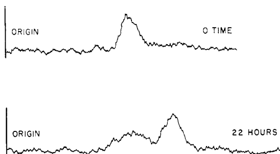
FIGURE 1: Scan of radioactivity along chromatographic chart of reaction mixture containing [2-^{14}\text{C}] CMP and malonyl hydrazide at pH 4.2 at zero time and 22 hr of incubation at 37^\circ . Solvent isopropyl alcohol-ammonia-water (7:1:2). The product has a lower mobility than the unreacted nucleotide.
