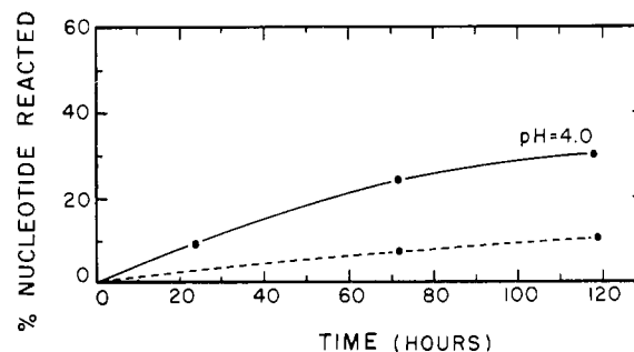
FIGURE 9: Reaction rate of CMP with DSBH. Reaction mixtures contained 2 \times 10^{-4} M 2\text{-}^{14}\text{C} -labeled CMP in 1 M DSBH at pH 4. The solutions were incubated at 37° and analyzed by electrophoresis at pH 7. An addition product with higher electrophoretic mobility is formed (solid line). At the same time a breakdown product indicated by an immobile peak (broken line) is also formed.
